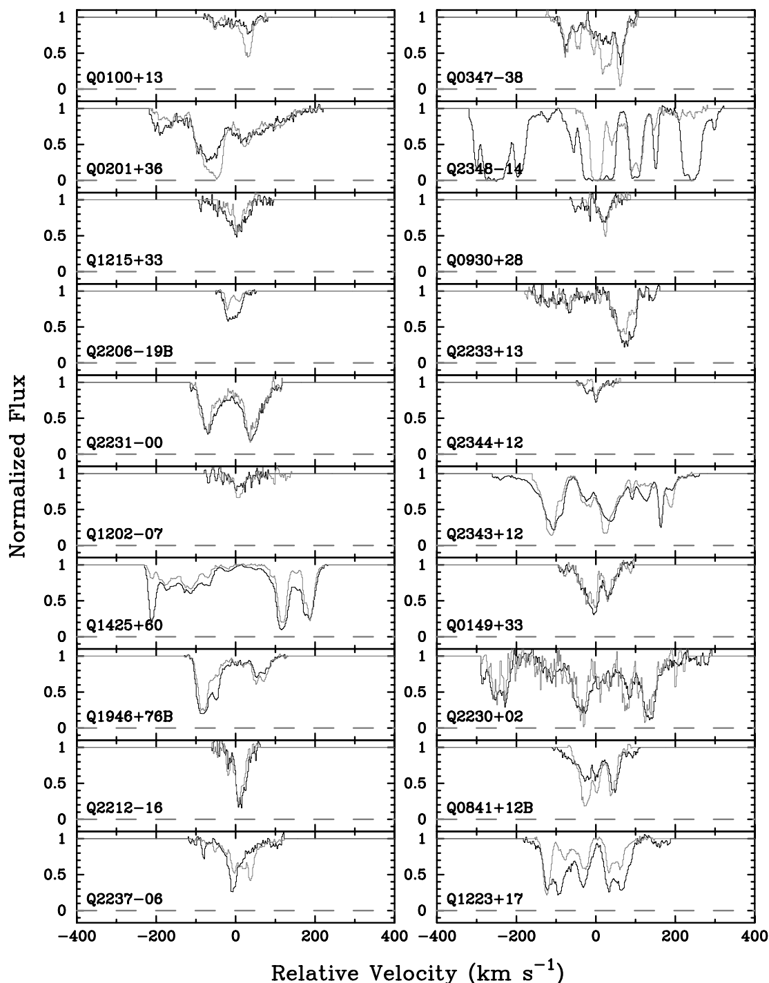
FIG. 4.—Velocity profiles of C IV ( dark lines ) and Si IV ( gray lines ) transitions for all damped Ly \alpha protogalaxies in Table 1 in which HIRES Si IV and C IV profiles have been measured. Velocity scale same as in Fig. 1.
