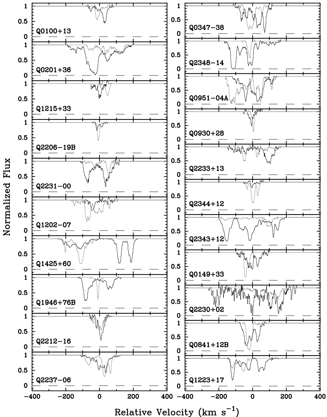
FIG. 2.—Velocity profiles of Si IV ( dark lines ) and low-ion ( gray lines ) transitions for all damped Ly \alpha protogalaxies in Table 1 in which HIRES Si IV and low-ion profiles have been measured. Velocity scale same as in Fig. 1.
