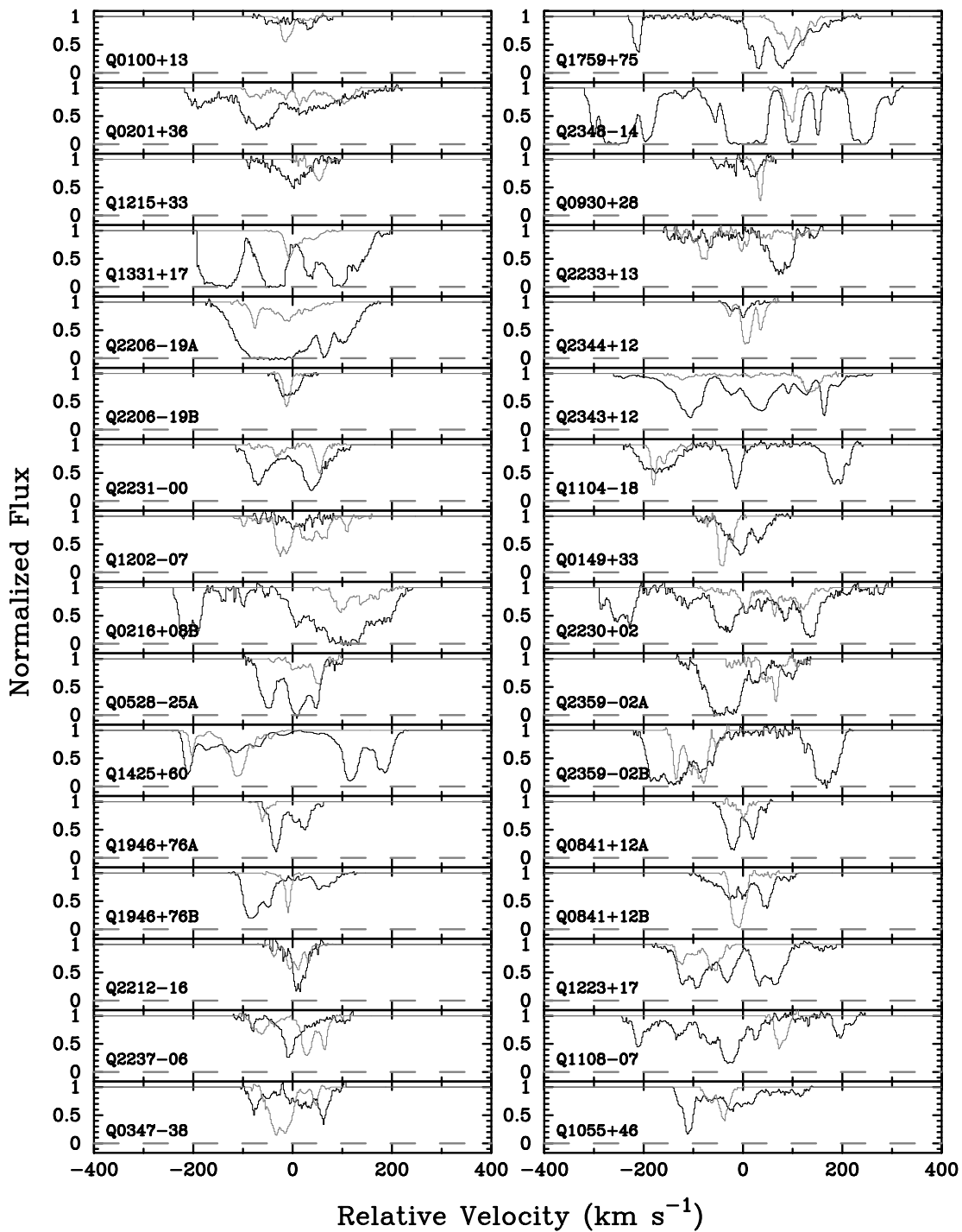
FIG. 1.—Velocity profiles of C IV (dark lines) and low-ion (gray lines) transitions for all damped \text{Ly}\alpha protogalaxies in Table 1 in which HIRES C IV and low-ion profiles have been measured. The velocity v = 0 corresponds the absorption redshift, z_{\text{abs}} , shown in the table.
