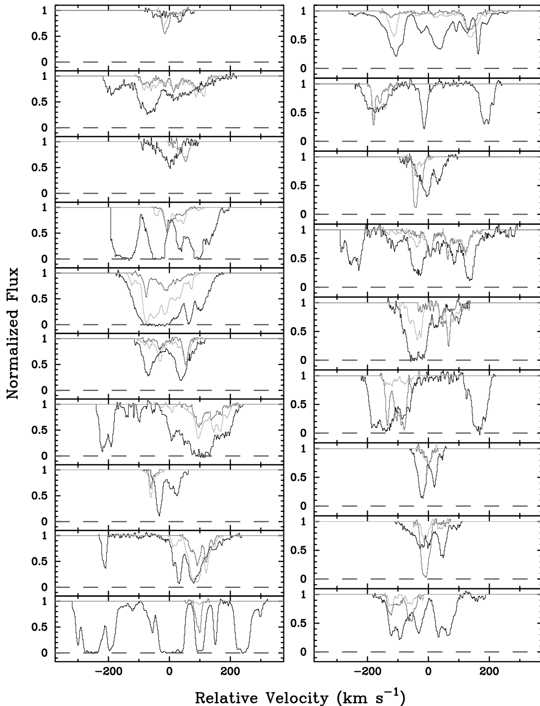
FIG. 5.—Velocity profiles of C IV (dark lines), Al III (light gray lines), and low-ion (medium gray lines) transitions for all damped \text{Ly}\alpha protogalaxies in Table 1 in which Al III, C IV, and low-ion profiles have been measured. Velocity scale same as in Fig. 1.
