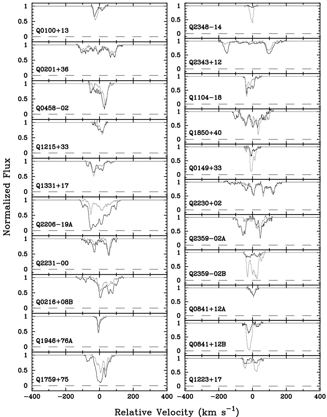
FIG. 3.—Velocity profiles of Al III (dark lines) and low-ion (gray lines) transitions for all damped \text{Ly}\alpha protogalaxies in Table 1 in which HIRES Al III and low-ion profiles have been measured. Velocity scale same as in Fig. 1.
