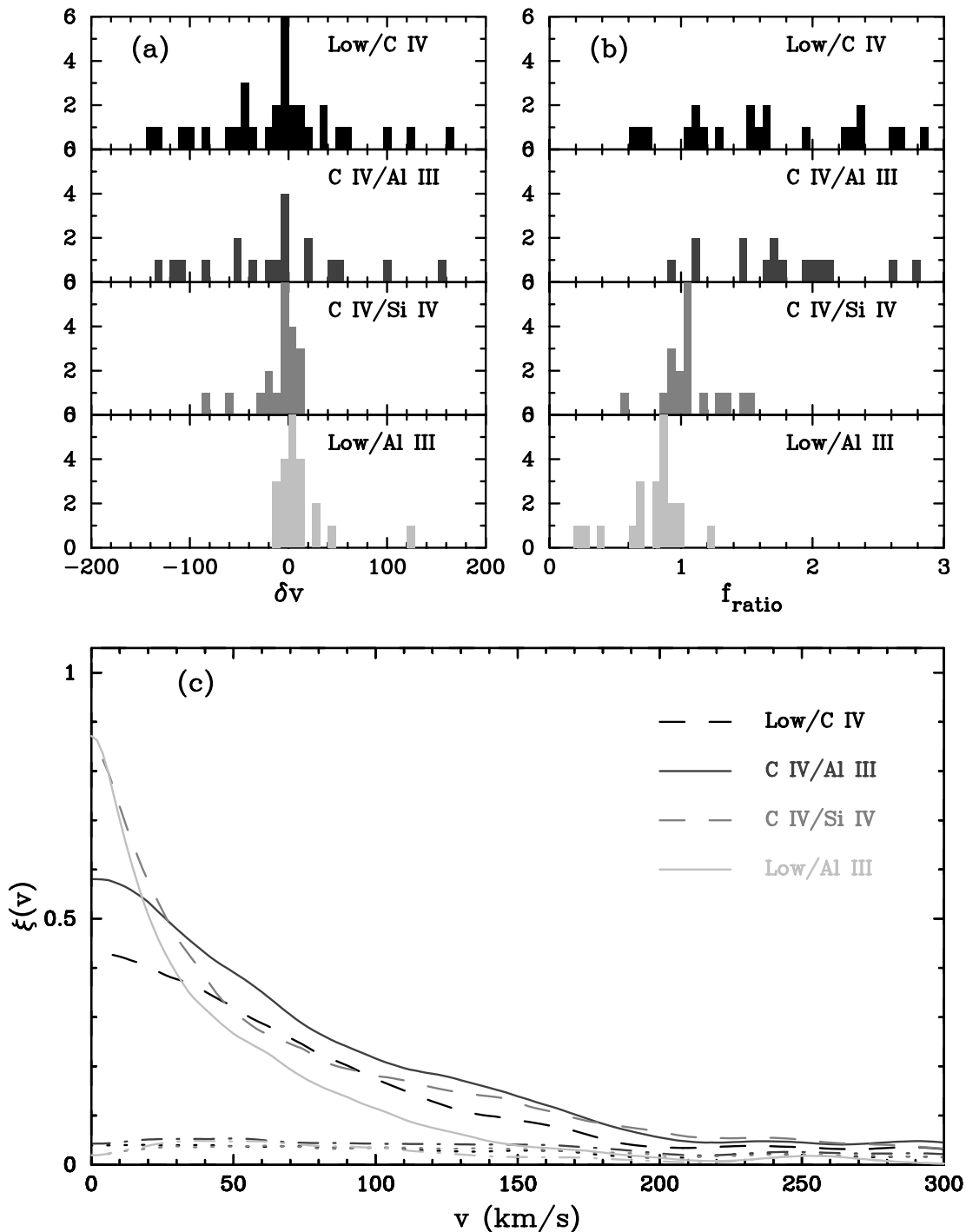
FIG. 7.—Empirical distributions of correlation test statistics (a) \delta v and (b) f_{\text{ratio}} , and (c) cross-correlation functions \xi_{ab}(v) for low-ion vs. C IV (dark dashed curve), C IV vs. Al III (dark solid curve), C IV vs. Si IV (light dashed curve), and low-ion vs. Al III (light solid curve) velocity profiles. Lower dashed curves show 1\sigma errors.
