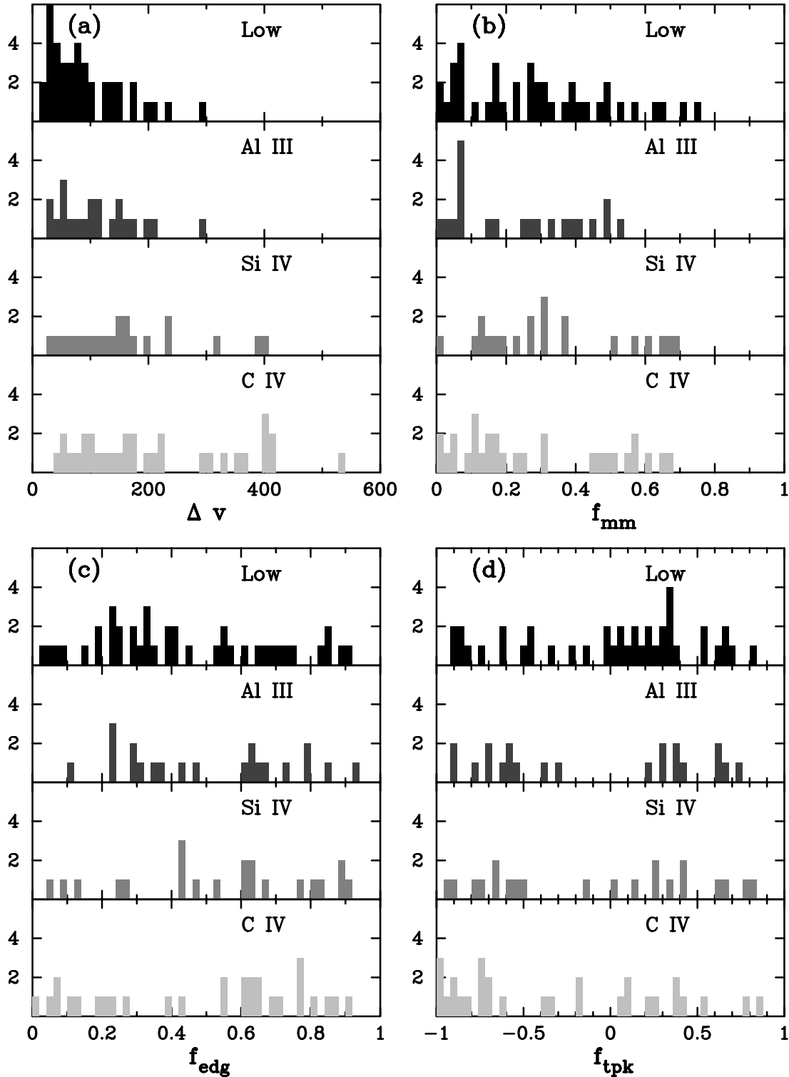
FIG. 6.—Empirical distributions of test statistics (a) \Delta v , (b) f_{\text{mm}} , (c) f_{\text{edg}} , and (d) f_{\text{tpk}} for low-ion, Al III, Si IV, and C IV velocity profiles
