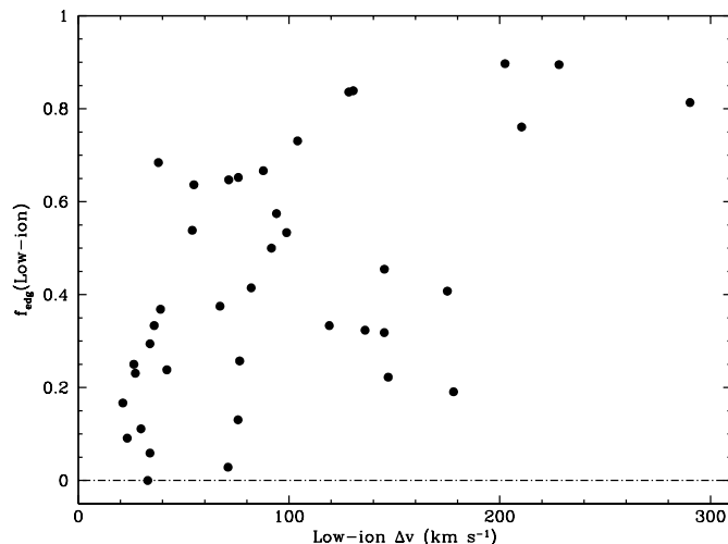
FIG. 9.—Plot of f_{\text{cdg}} vs. \Delta v for low-ion profiles in Table 1
