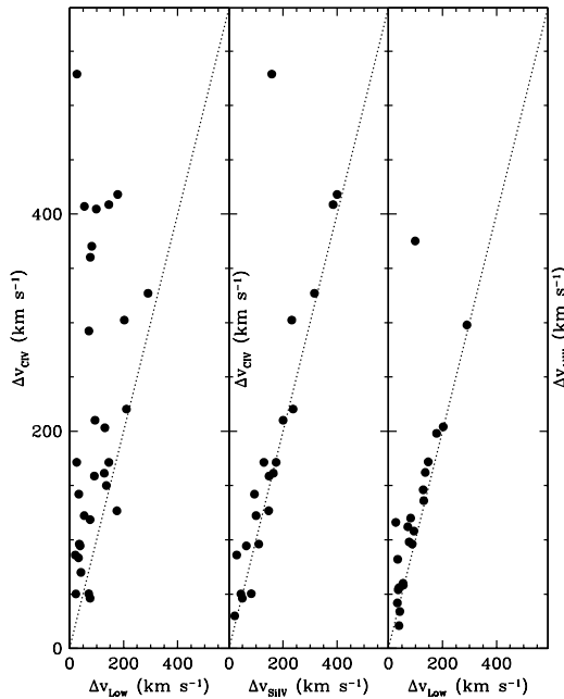
FIG. 8.—Plots of \Delta v for the ion pairs (a) C IV vs. low-ion, (b) C IV vs. Si IV, and (c) Al III vs. low-ion.
